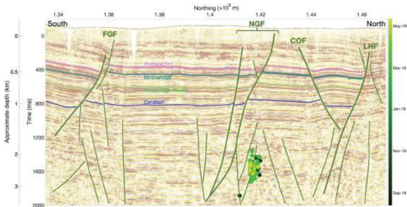
▲ Figure 6. 2D seismic section along profile TWLD-90-15 (Fig. 2) showing interpreted faults (green lines), geological formations, together with the projected positions of double-difference 40 relocated earthquakes from this study. The color of each event denotes the time that each event occurred. COF, Collendean fault; FGF, Faygate fault; LHF, Leigh fault; NGF, Newdigate fault. An uninterpreted version of this section is shown in © Figure S13. The color version of this figure is available only in the electronic edition.
